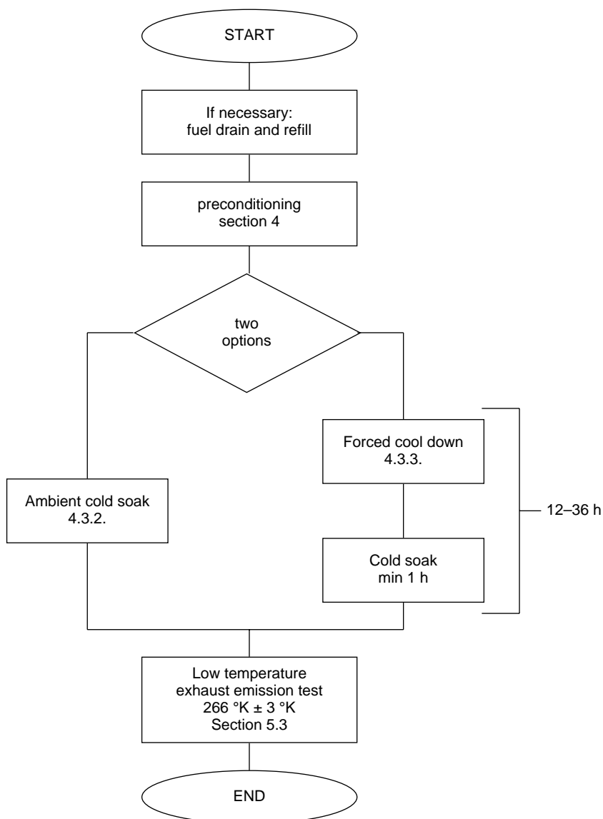
Procedure for low ambient temperature test
